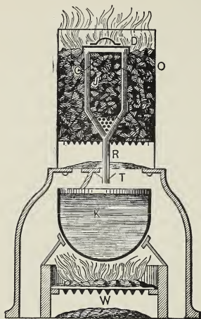
FIG. 9.—Andrès' Apparatus.
